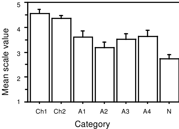
Fig. 7. Mean musical well-formedness ratings for the fragments in the 7 categories obtained in Experiment 2a. Ch1 = activation of a triad; Ch2 = activation of a seventh chord; A1 = immediate anchoring; A2, A3, A4 = anchoring with one, two, or three intermediate tones, respectively; N = does not form a percept.
